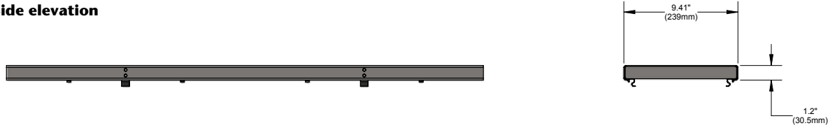
Side elevation
