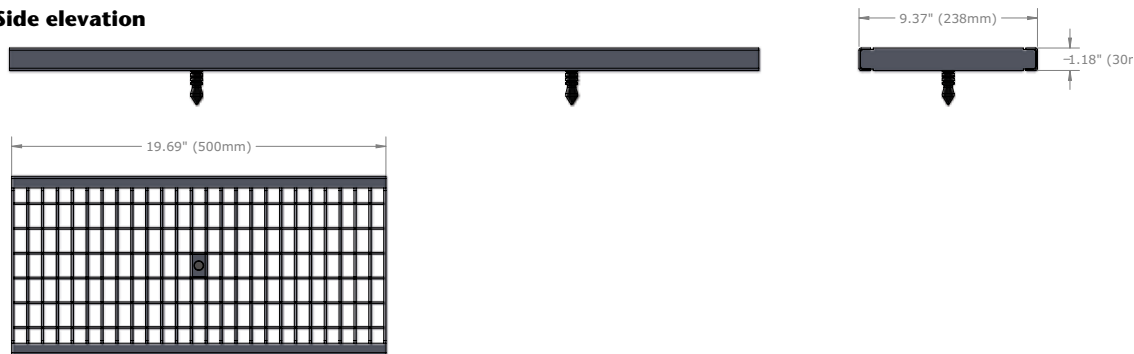
Side elevation
