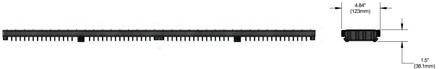
Side elevation
