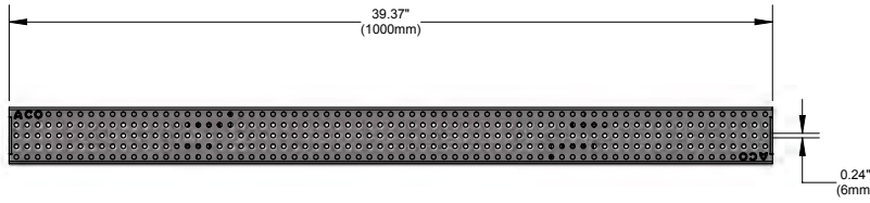
Plan view
