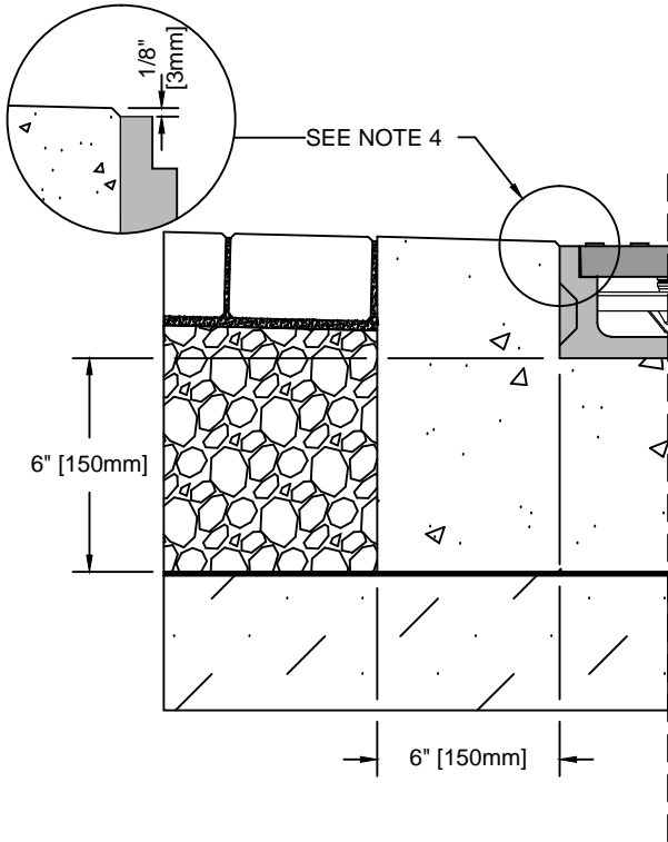
STANDARD INSTALLATION
